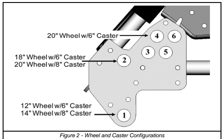
Figure 2 - Wheel and Caster Configurations
