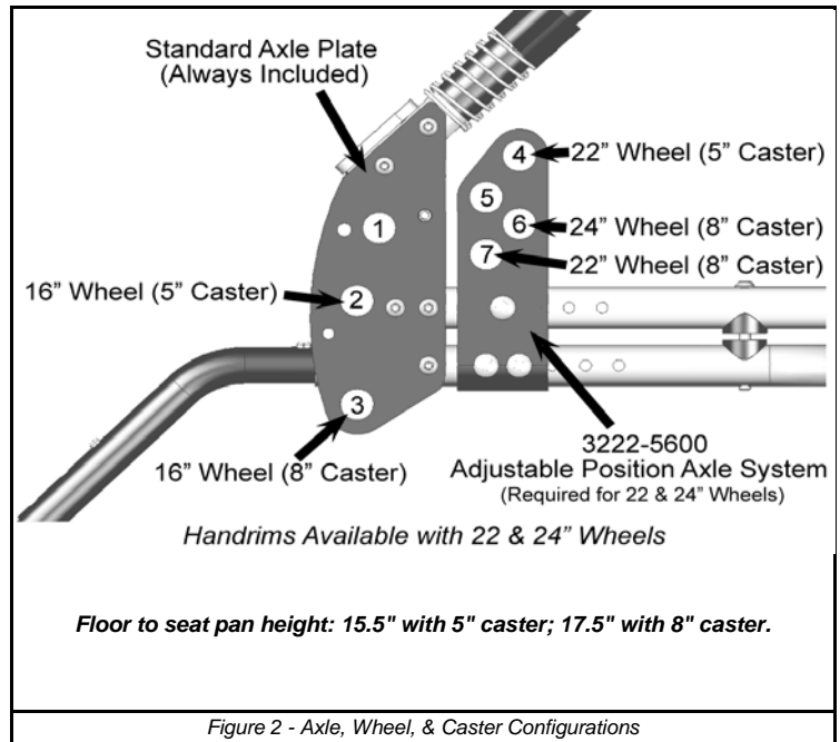
Figure 2 - Axle, Wheel, & Caster Configurations
